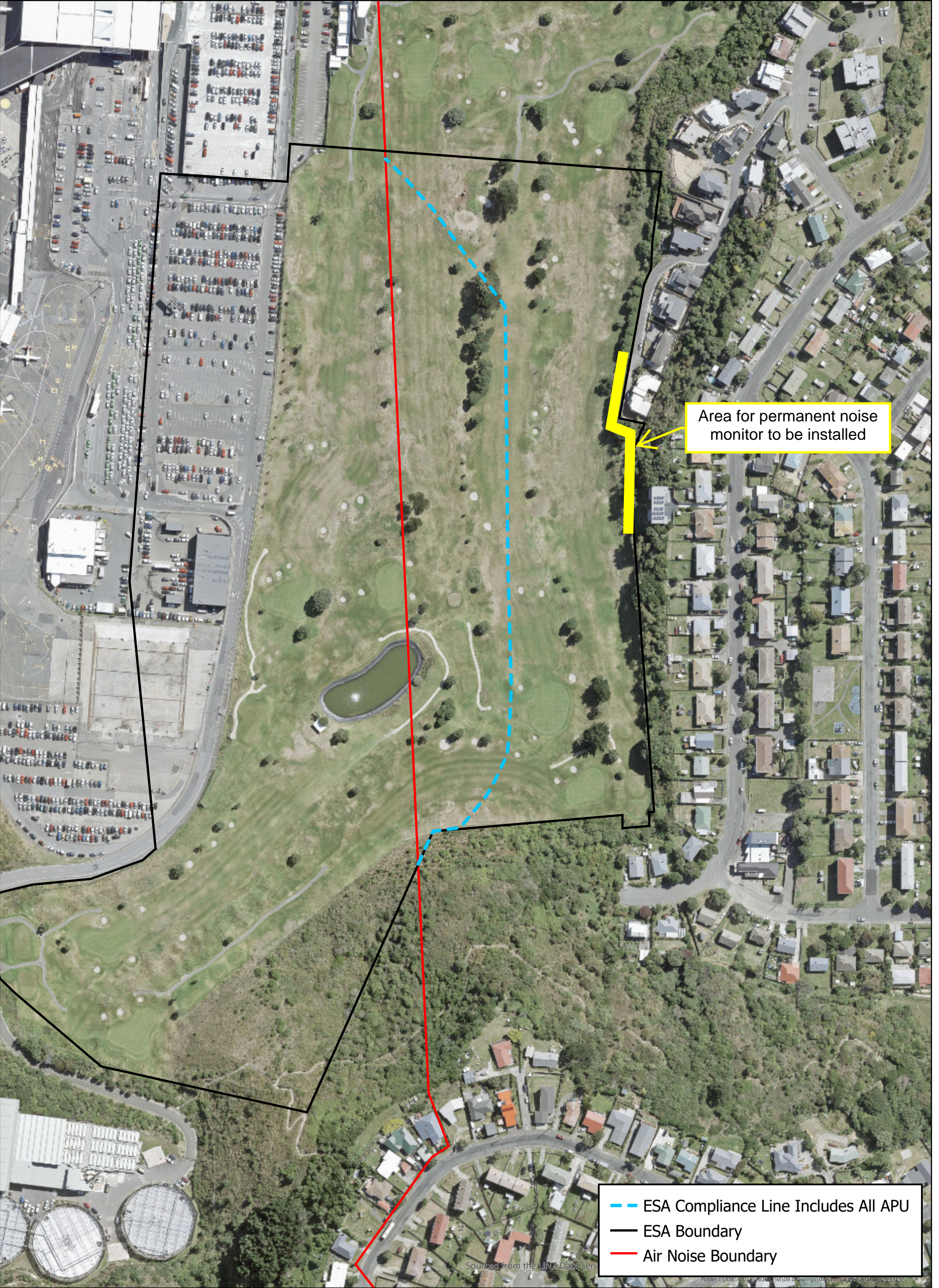
Figure 1: Wellington Airport ESA Designation Compliance Line Adjustments for APUs
