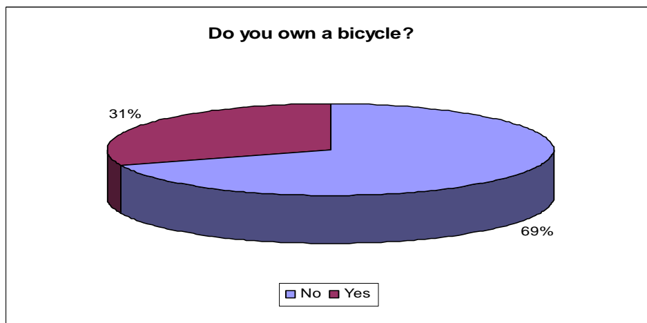
Figure 38: Bicycle ownership
